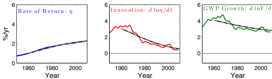
Figure 7. Black, gray-dashed lines: hindcasts starting in 1960 of the global rate of return \eta = Y / \int_0^t Y dt' , innovation rates d \ln \eta / dt , and the GWP growth rate d \ln Y / dt = \eta + d \ln \eta / dt . Hindcasts are derived from Eq. (16) assuming an average rate of technological change of 5.1 % yr -1 (dashed gray lines) derived from conditions observed in the 1950s. Solid colored lines: observed decadal running means. Hindcast values in 1960 represent persistence values shown in Table 1.
