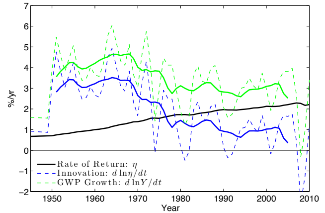
Figure 4. Time series of the rate of return, innovation, and the GWP growth rate, evaluated at global scales and expressed in percent per year. Solid lines represent a running decadal mean (see Garrett, 2014, for methods).
